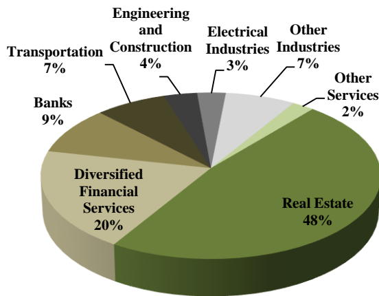
Figure 5: Value Traded
