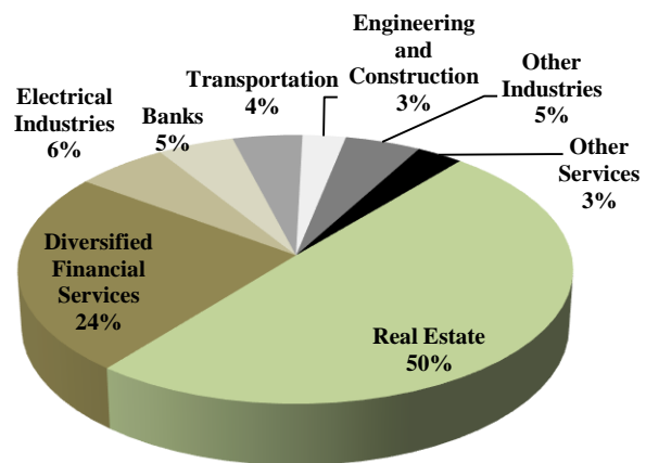
Figure 5: Trading Volume
